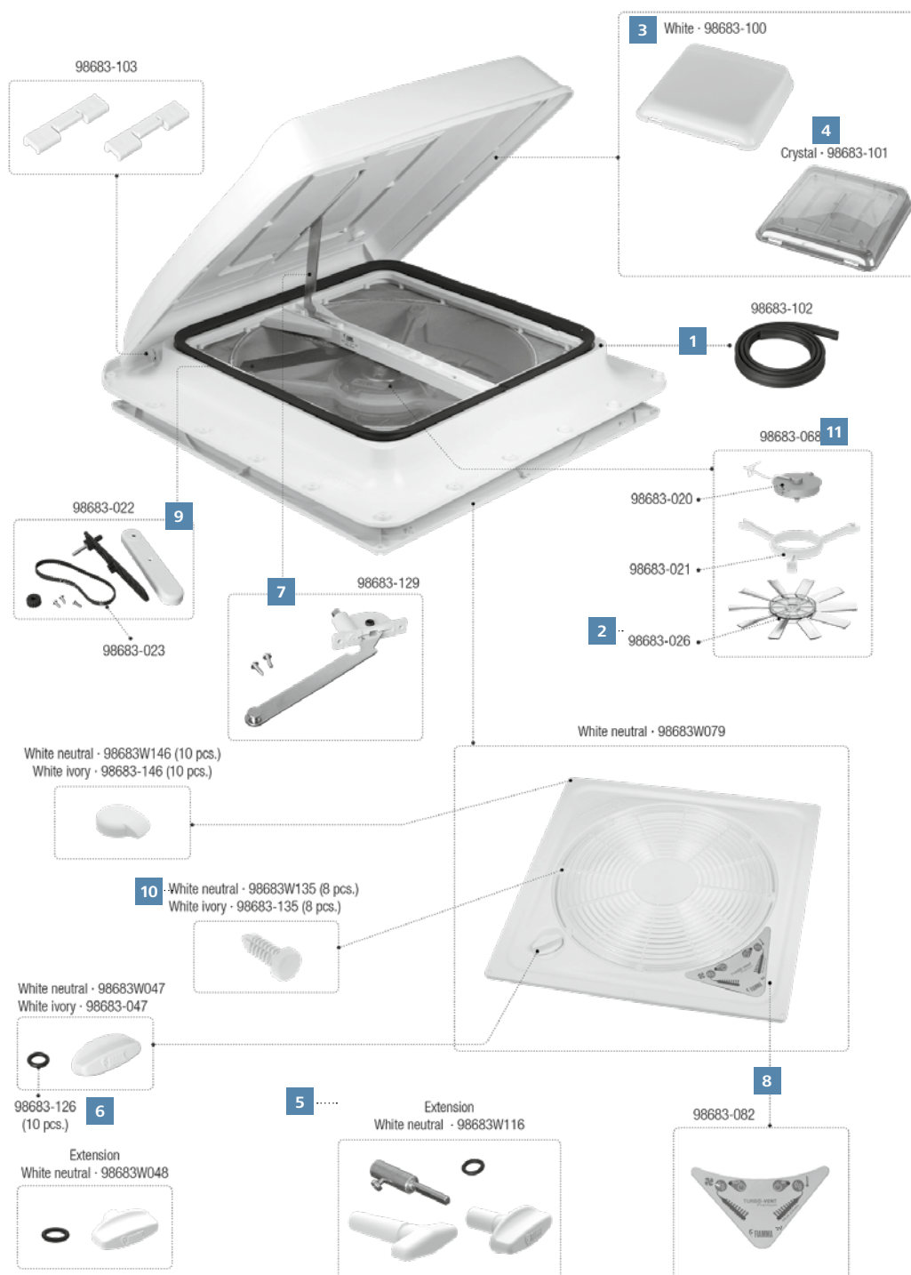
Dachhaube Turbo Vent Premium crystal 03624H02D 206/430
